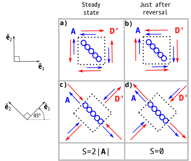
Fig. 2 Tensors' components for \mathbf{A} and \mathbf{D}' and S values are displayed at steady state and just after reversal for 2D simple shear. The components are showed respect to a coordinate system pointing in the horizontal and vertical direction, and respect to a second coordinated system rotated 45^\circ .
