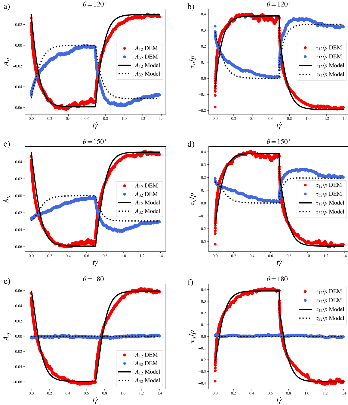
Fig. 6 Comparison between model and DEM simulations of the off-diagonal components of the fabric and normalized shear stress during transients. The angles \theta of the shear-rate rotation corresponds to [120^\circ, 150^\circ, 180^\circ] . Figures a), c), and e): fabric components comparison. Figures b), d), and f): comparison of the normalized shear stress components.
