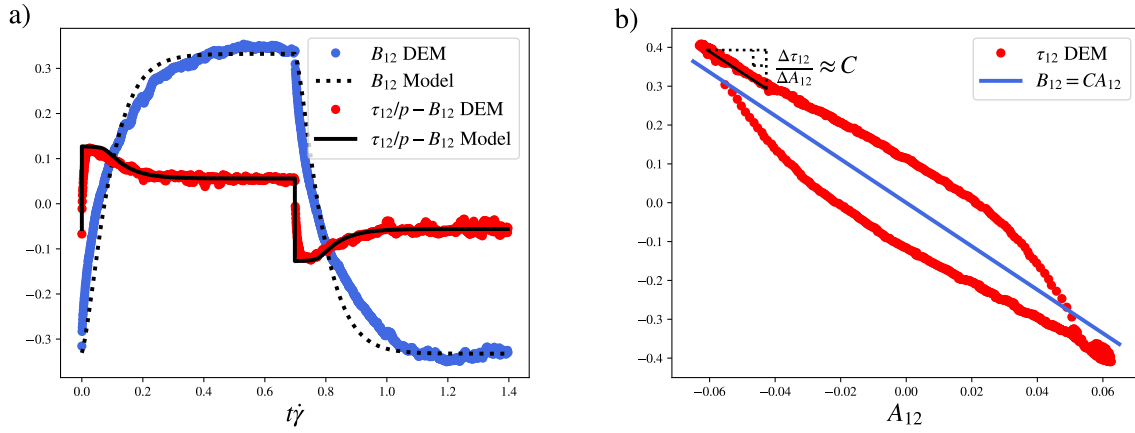
Fig. 8 Analysis of the stress evolution during the reversal case. a) Backstress and isotropic flow resistance. b) Shear stress component \tau_{12} versus fabric component A_{12} .
