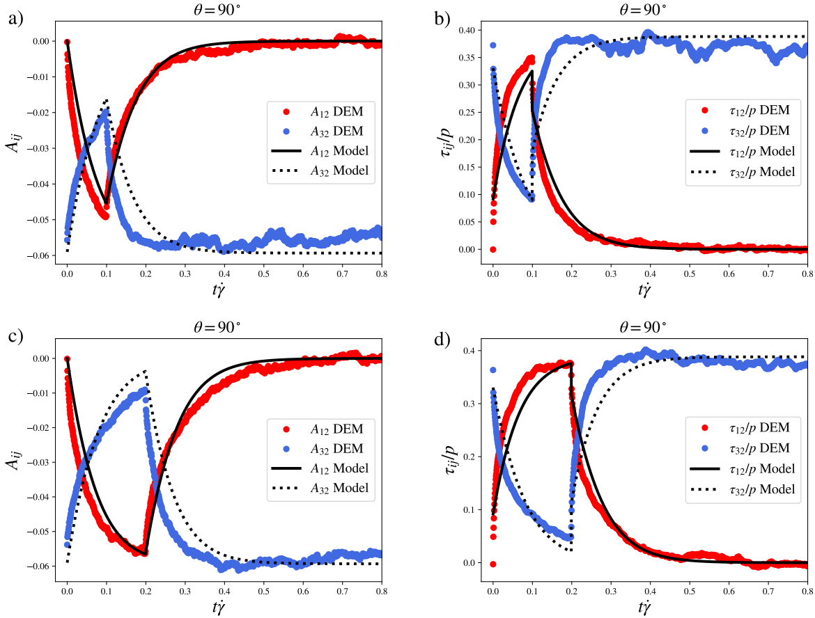
Fig. 7 Comparison between model and DEM simulations of the off-diagonal components of the fabric and normalized shear stress during transients for \theta = 90^\circ rotated at small strains. Figures a) and b) show the fabric and normalized shear stress components for a change in the shear orientation at t\dot{\gamma} = 0.1 , while for figures c) and d) the change is when t\dot{\gamma} = 0.2 .
