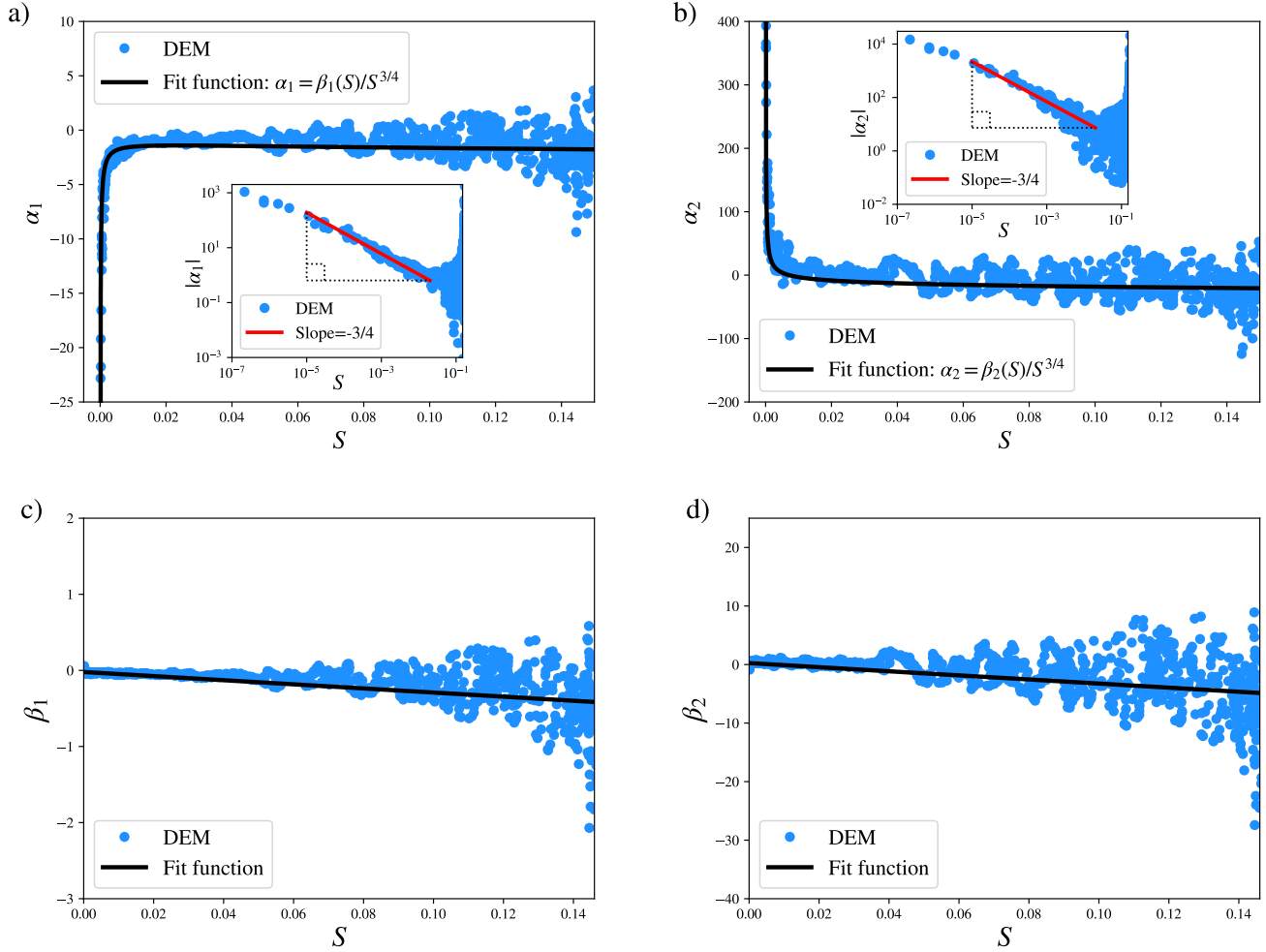
Fig. 3 Light blue points in figures a) and b) correspond to the value of the \alpha_i coefficients from Eq. 9 versus the S hardening variable obtained from a DEM reversal (insets show the absolute values of \alpha_i on a logarithmic scale). Fit functions \alpha_i(S) are shown with solid lines. Light blue points in figures c) and d) corresponds to the \beta_i coefficients from equation 13 versus the S hardening variable from the DEM reversal while solid black lines represent linear fits.
