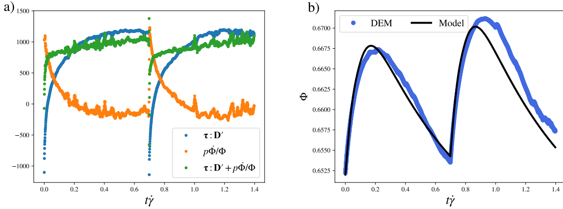
Fig. 9 (a) DEM data comparing the work-rate due to shear (blue), the work-rate due to volume change (orange), and the total work-rate \sigma : D = \tau : D' + p\Phi/\Phi (green) over a forward-reversal cycle in the \theta = 180^\circ case. (b) The packing fraction over the same time range obtained in DEM and from the dilation model, equation 18.
