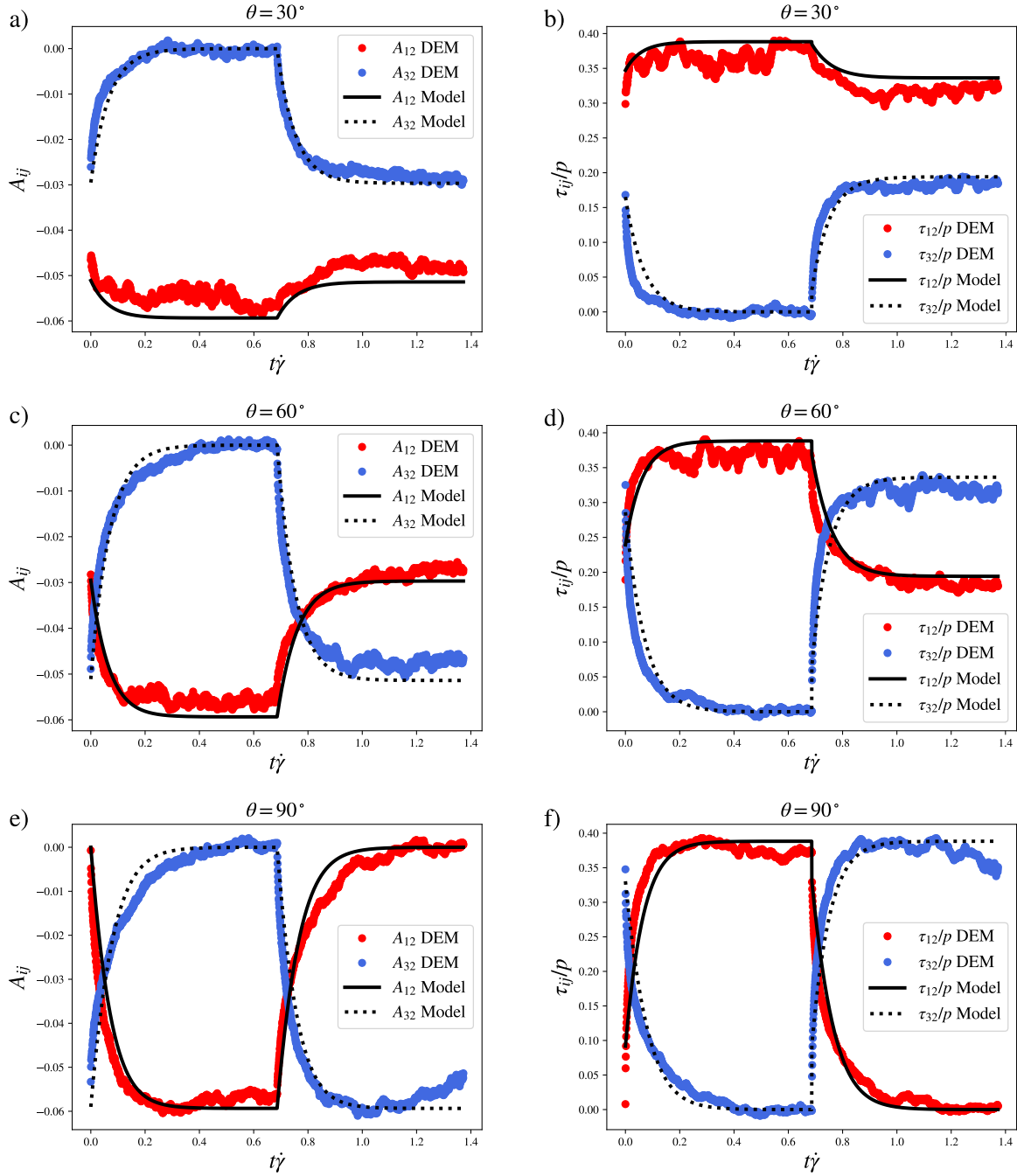
Fig. 5 Comparison between model and DEM simulations of the off-diagonal components of the fabric and normalized shear stress during transients. The angles \theta of the shear-rate rotation corresponds to [30^\circ, 60^\circ, 90^\circ] . Figures a), c), and e): fabric components comparison. Figures b), d), and f): comparison of the normalized shear stress components.
