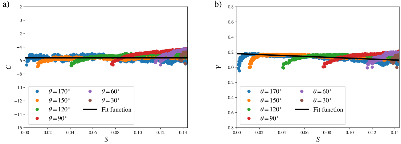
Fig. 4 DEM results and fit functions for the shear stress model proposed in the present work (Eq. 14). a) Backstress parameter C , b) Yield function Y(S) .
