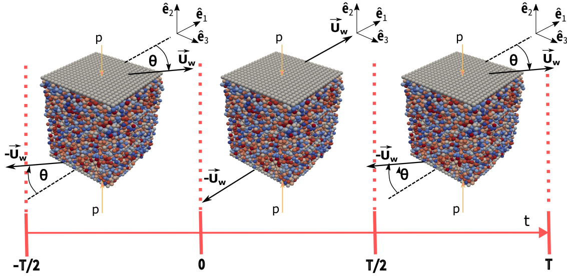
Fig. 1 Numerical setup. The red line corresponds to time, with tick marks indicating changes to the walls' velocities. The part from t = 0 to t = T corresponds to one period. A half period at the beginning was also simulated. The different walls' velocities for each part of the periodic cycle are shown. From t = 0 to t = T/2 , the velocity of the top wall is in the \hat{e}_1 direction, while the bottom wall moves in the opposite direction. At t = T/2 the direction of the walls' velocities are rotated instantaneously by an angle \theta in the plane perpendicular to \hat{e}_2 until t = T . Note that there is a previous walls' rotation at t = 0 to produce a periodic process.
